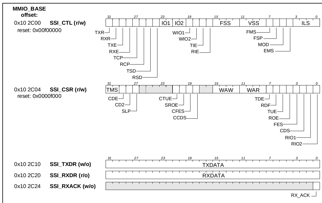
Figure 17-10. SSI MMIO registers.
