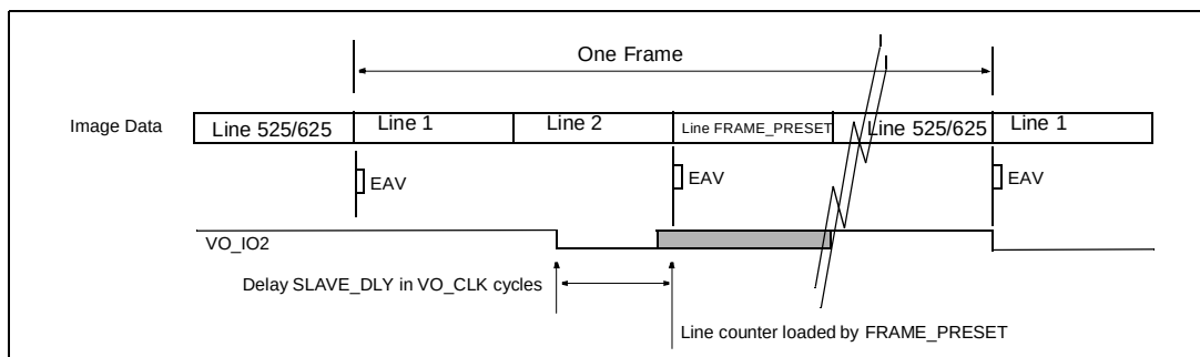
Figure 7-16. Genlock mode.
