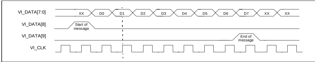
Figure 6-17. VI message passing signal example.
