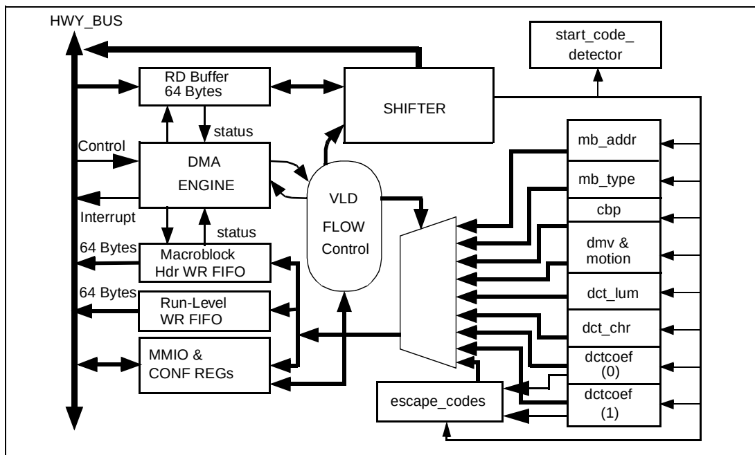
Figure 15-1. VLD block diagram
