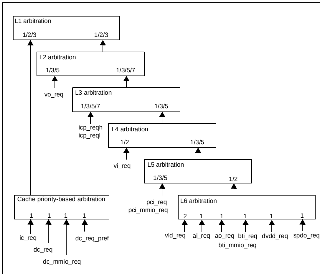
Figure 20-5. Arbitration architecture
